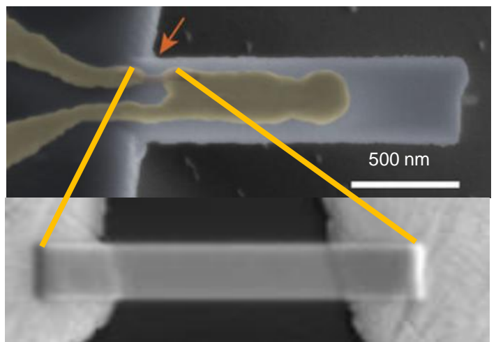
Fig.2.: Strain Nanosensor (orange arrow) 3D-printed on a cantilever that can be attached to the osmotic pressure chamber membrane
