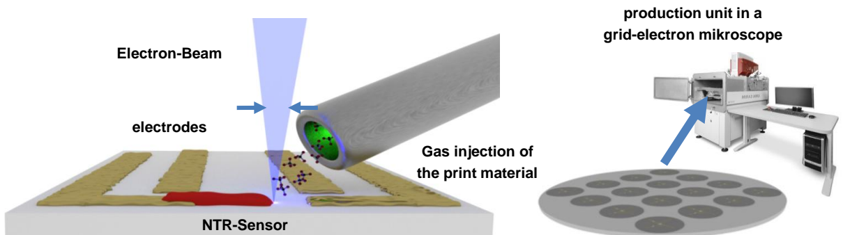
Fig.4.: Manufacturing of the nanosensors by means of the 3D-Nanosense® printing process (CantiMed)
